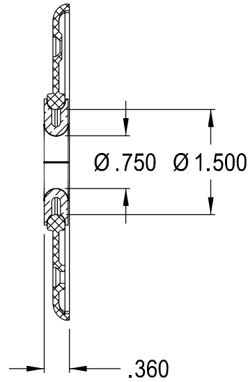
1.000" BUSHING FOR 1-GANG
